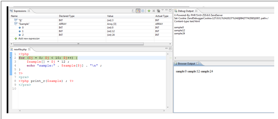
Figure 16-2. The debugger in action with watch expressions defined
